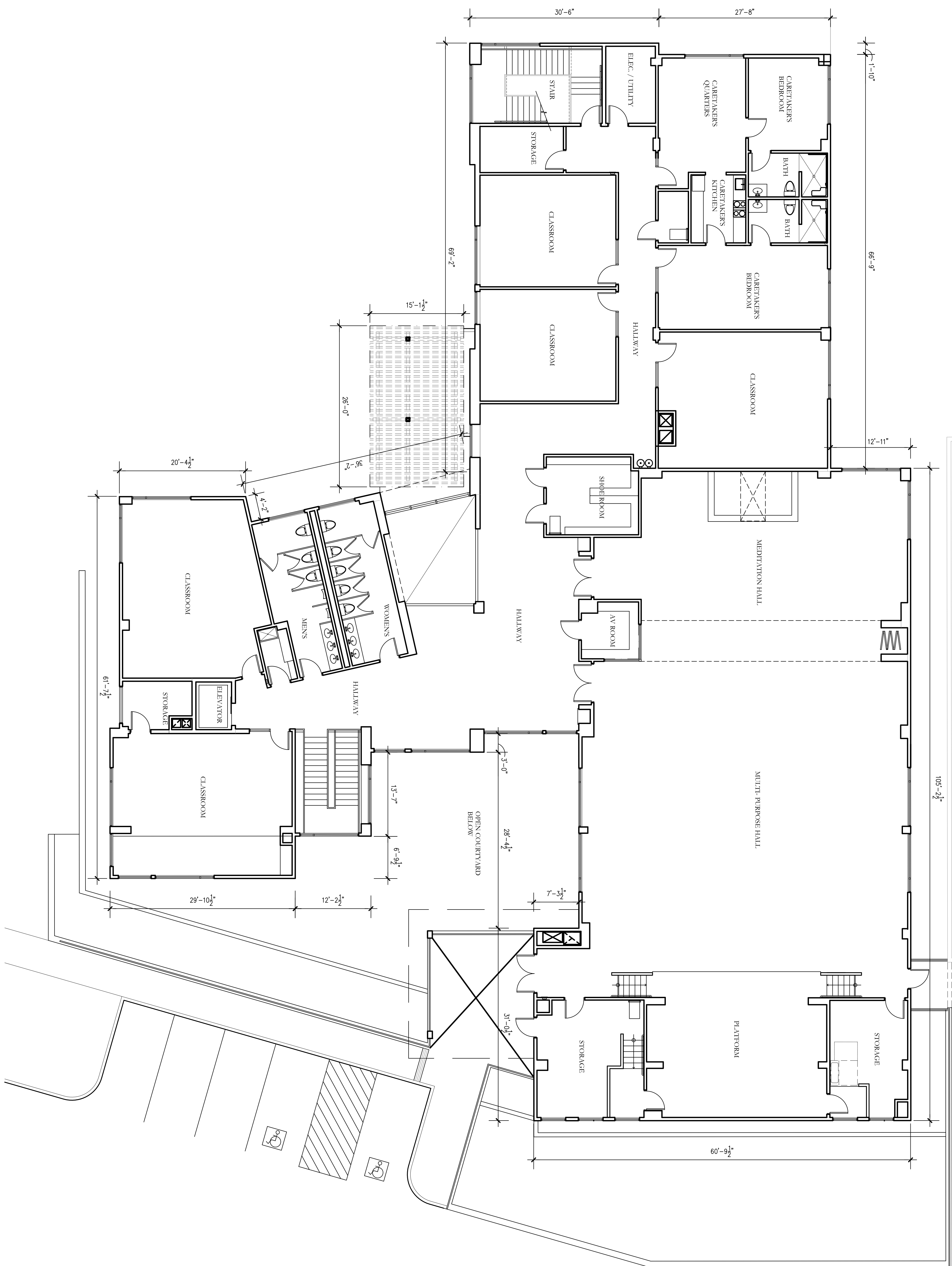
1 OVERALL FLOOR PLAN - UPPER LEVEL SCALE: 1/8" = 1'-0" AREA = 13,232 S.F.
